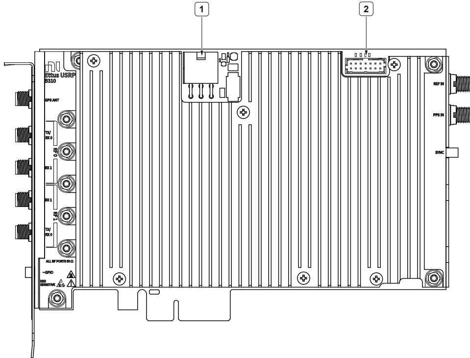
Figure 1. USRP B310 (PCIe) Front/Rear Panels
